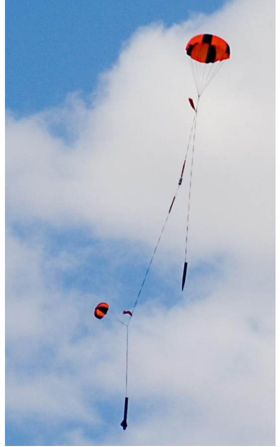
Mike Garrett's "Dark Matter" flew nicely to 5500' on a K500RL motor. The rocket is based on a Mad Dog DD kit.
